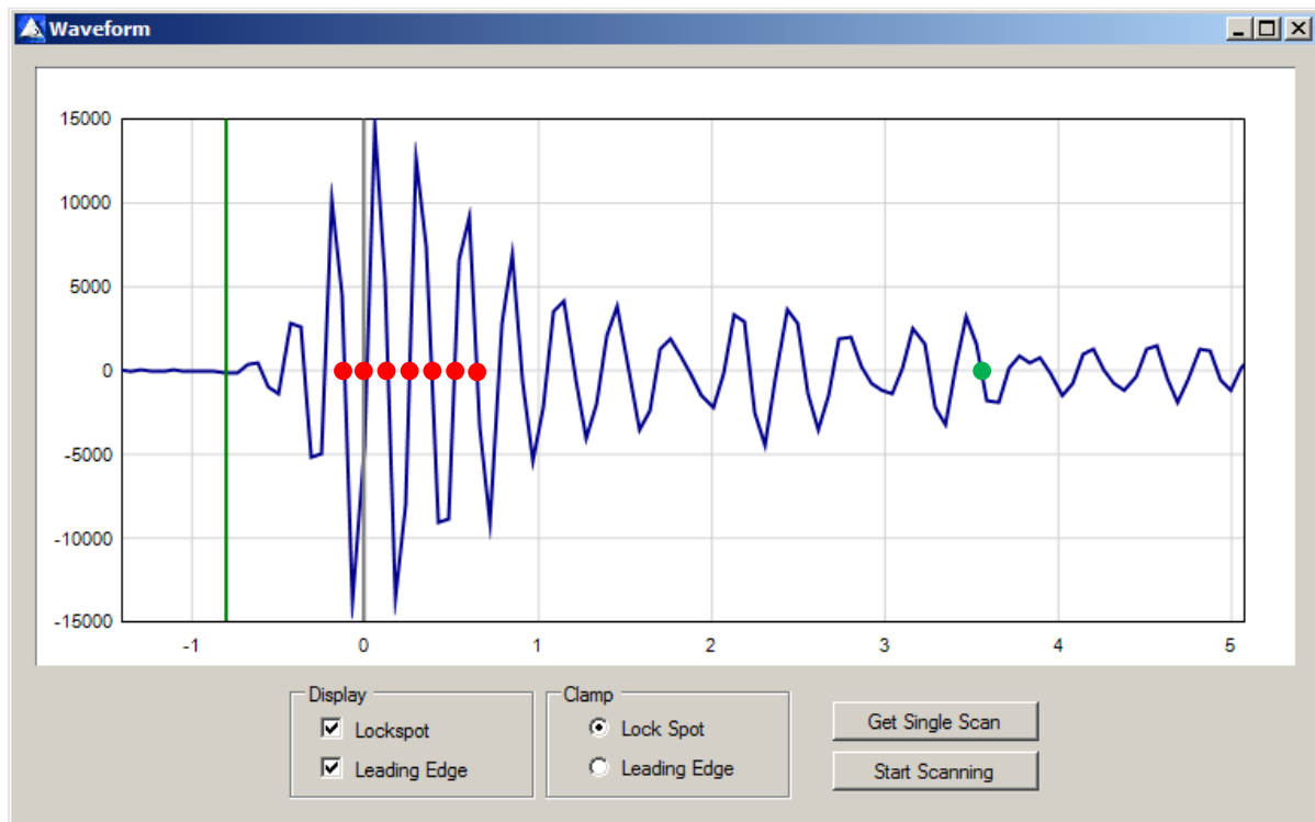
Figure 6: Sample captured waveform showing potential radio lock spots
