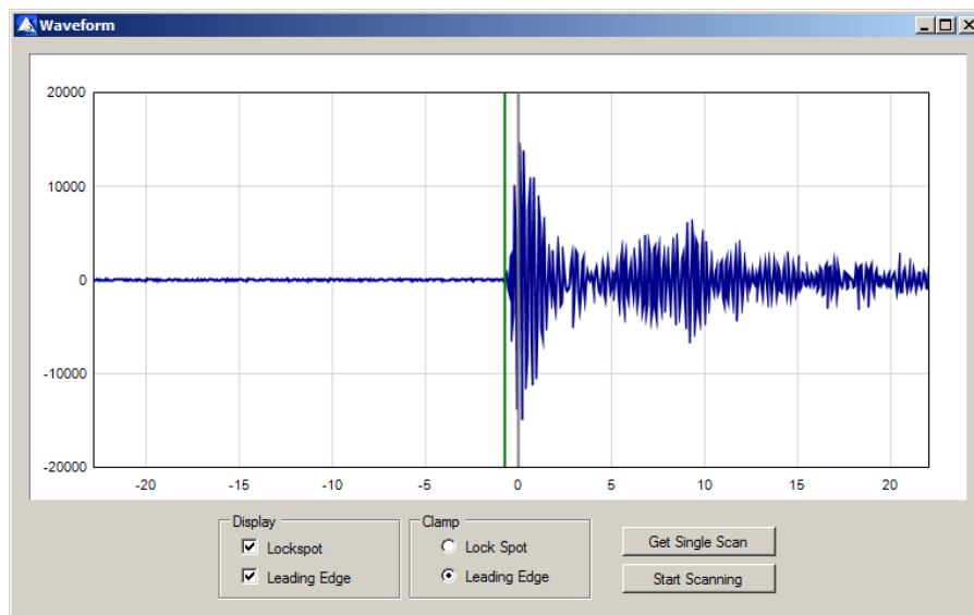
Figure 8: Typical waveform scan
